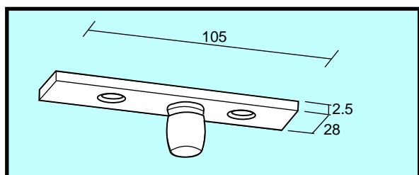
Pivot 12.5/15mm with fixing plate
