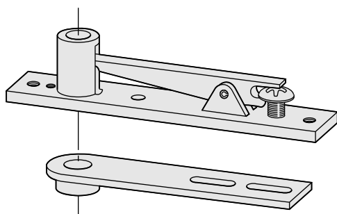
RETRACTABLE TOP CENTRE
