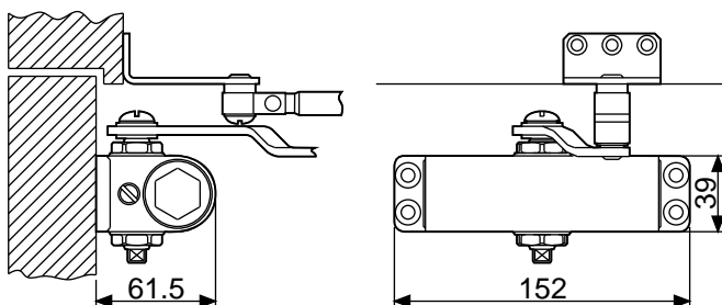
L - TYPE TRANSOM BRACKET(902)
