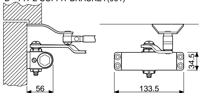
D - TYPE SOFFIT BRACKET(901)
